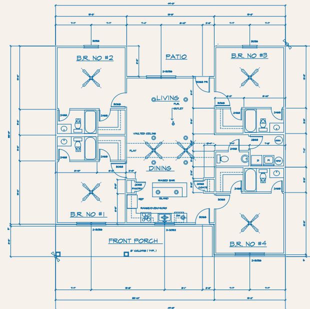
Floor Plan C
