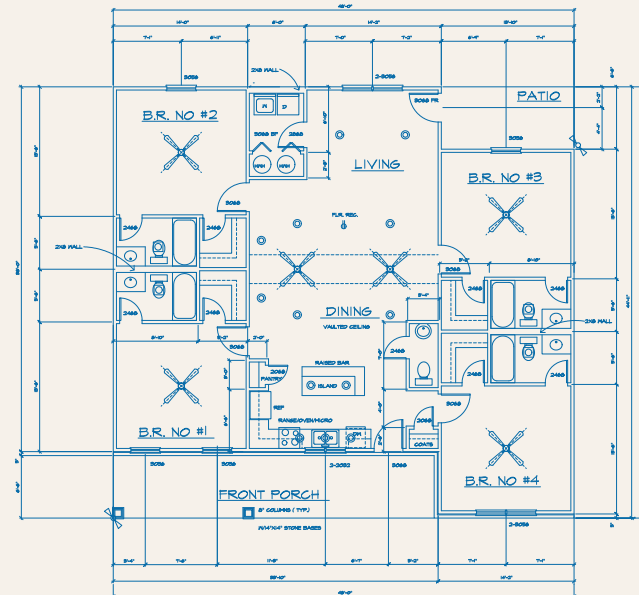
Floor Plan B
